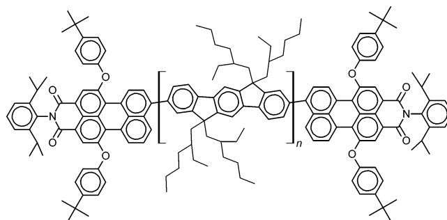
Figure 1. Molecular structure of \alpha,\omega -bis( N -(2,6-diisopropylphenyl)-1,6-bis-(4- tert -butylphenoxy)-3,4-dicarbonylacidimide-9-perylene-poly-2,8-(6,6,12,12-tetraethylhexyl)indenofluorene (PEC-PIFTEH).
